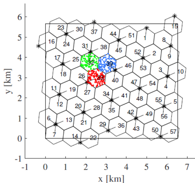
Figure 7: Synthetic scenario
