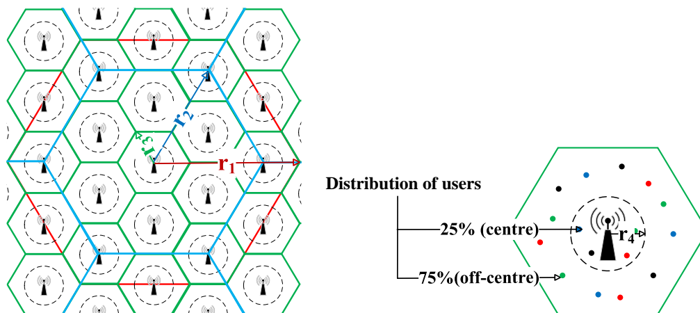
Figure 2: Network layout for the reference scenario (r_1=1.6 \text{ km}, r_2=1.2 \text{ km}, r_3=0.4 \text{ km}, r_4=0.05 \text{ km})
